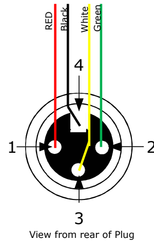
View from rear of Plug
