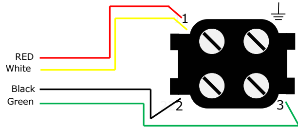
RED and Yellow to terminal 1. Black to terminal 2. Green to terminal 3. View from rear of plug.
