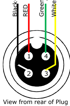
View from rear of Plug
