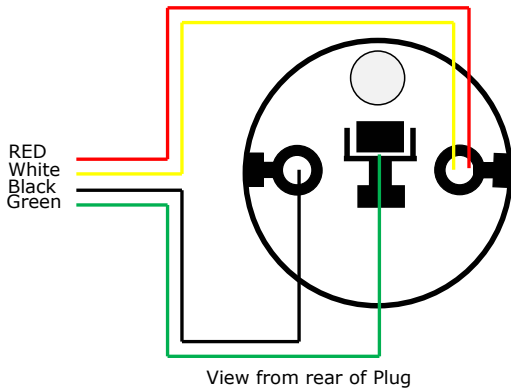
View from rear of Plug
