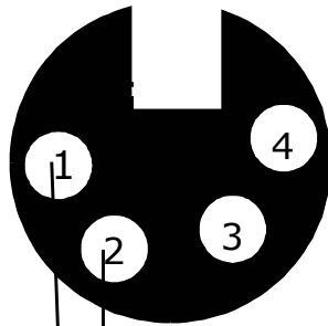
4 Pin XLR View from Rear
